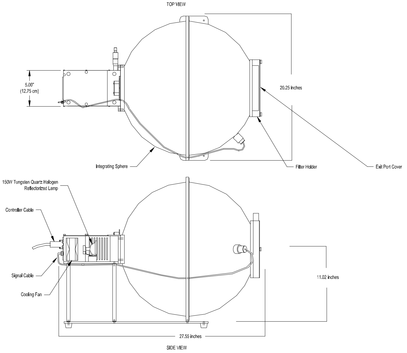
OL 455-18 Integrating Sphere Calibration Source
