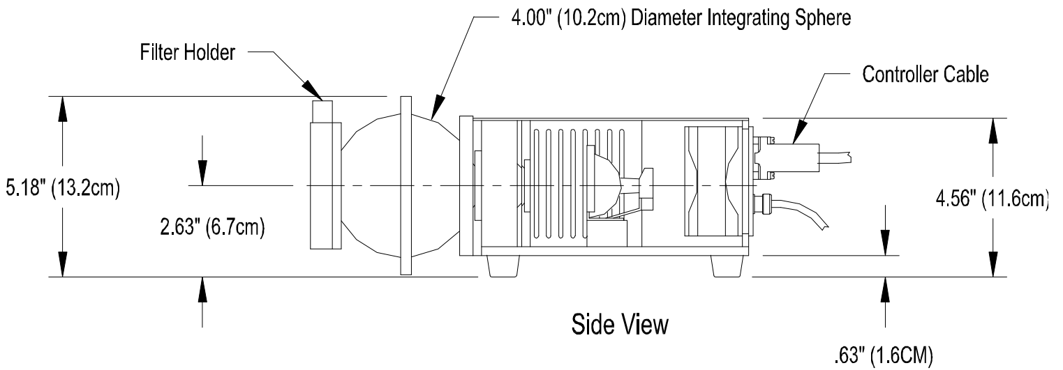
OL 455-4 Integrating Sphere Calibration Source
